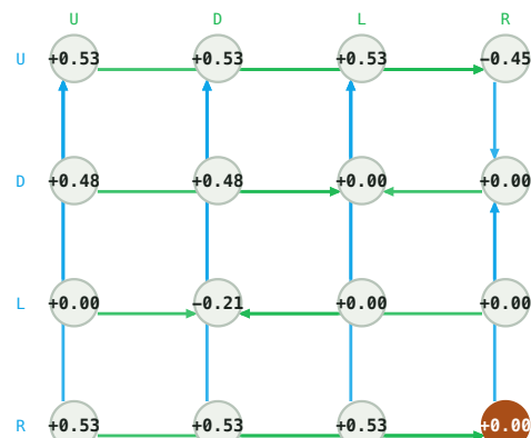
Q matrix -- (1, 0, 0, 1, 0)
