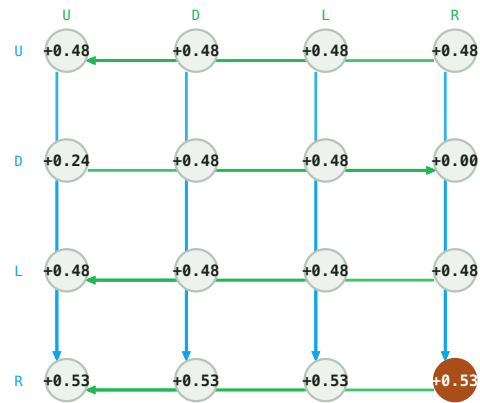
Q matrix -- (0, 2, 0, 0, 0)
