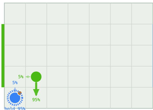
The corner duel -- (0,0) and (1,1)
