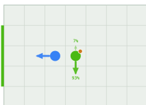
[4] 12 states
