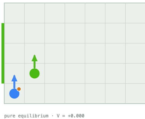
deterministic -> pure
