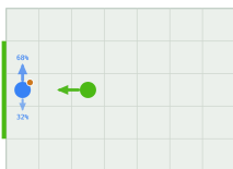
[8] 2 states
