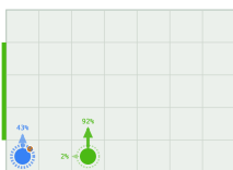
[6] 4 states
