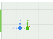
[2] 24 states
