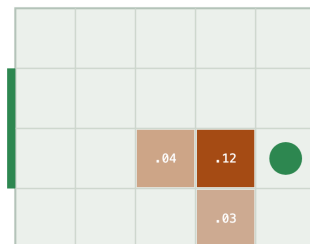
random
