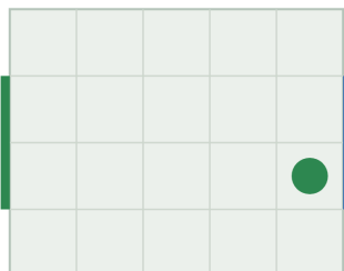
coinflip
