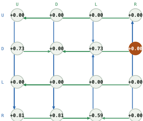
Q matrix -- (4, 3, 5, 3, 0)
