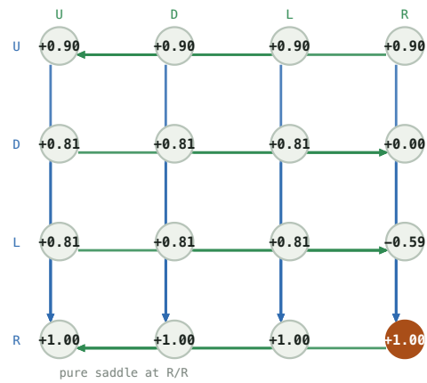
Q matrix -- (6, 1, 4, 1, 0)
