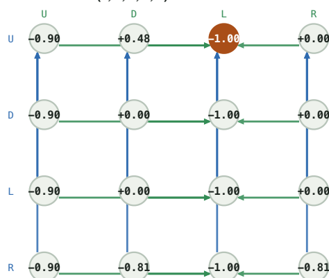
Q matrix -- (0, 0, 0, 1, 1)
