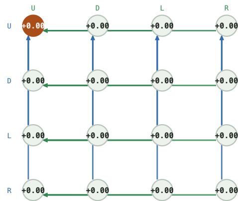
Q matrix -- (0, 0, 2, 0, 0)
