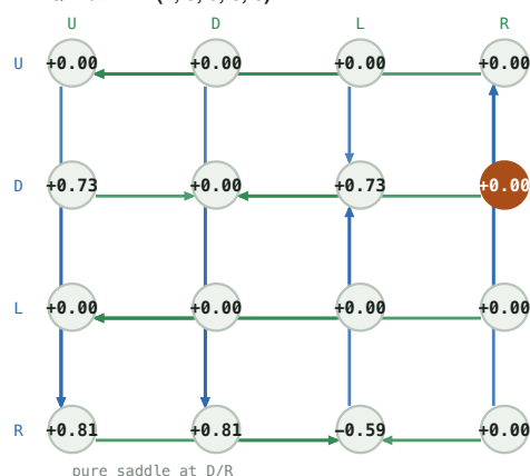
Q matrix -- (4, 3, 5, 3, 0)
