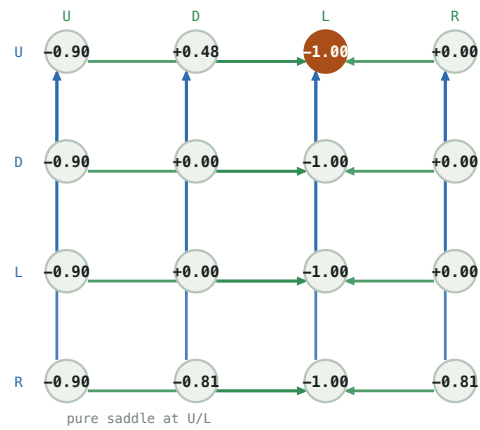
Q matrix -- (0, 0, 0, 1, 1)
