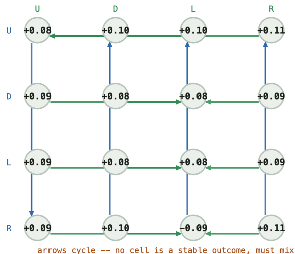
Q matrix -- (0, 0, 2, 0, 0)
