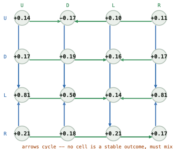
Q matrix -- (1, 1, 1, 0, 1)
