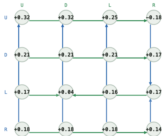
Q matrix -- (1, 1, 2, 0, 1)
