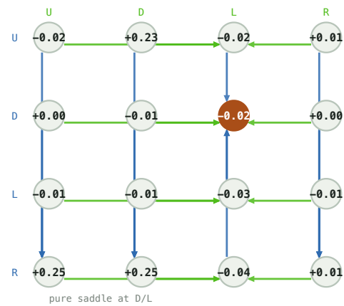
Q matrix -- (1, 1, 2, 1, 0)
