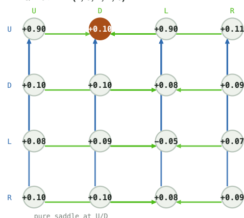
Q matrix -- (4, 0, 4, 1, 0)
