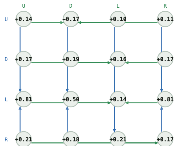
Q matrix -- (1, 1, 1, 0, 1)
