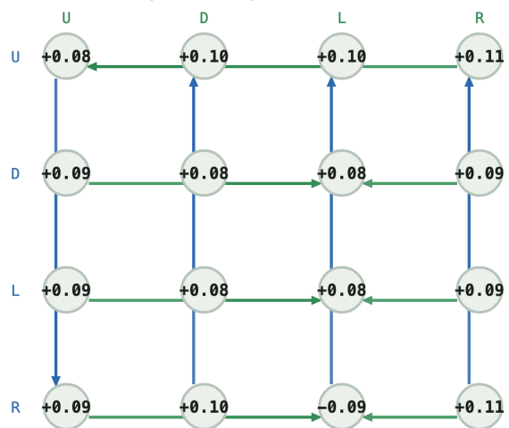
Q matrix -- (0, 0, 2, 0, 0)
