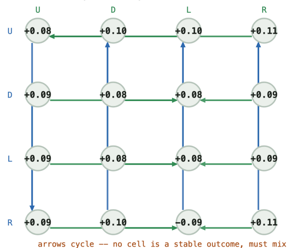
Q matrix -- (0, 0, 2, 0, 0)
