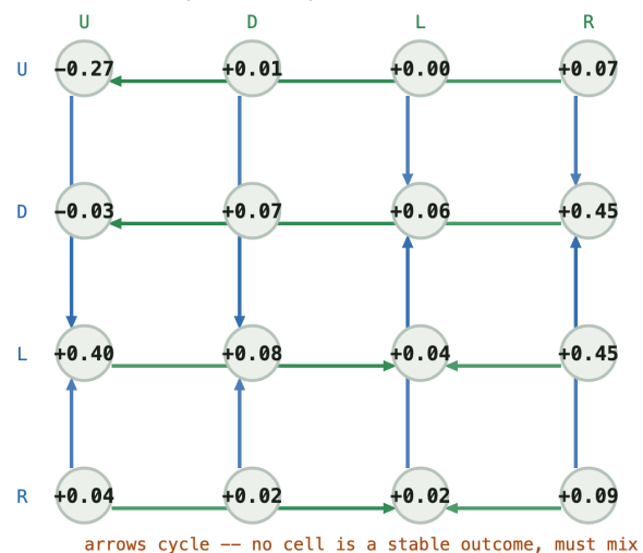
Q matrix -- (1, 3, 1, 4, 1)
