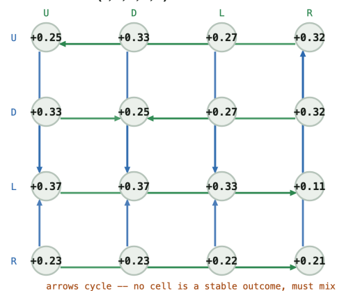
Q matrix -- (0, 2, 2, 2, 1)
