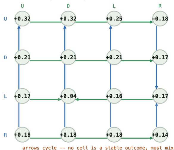
Q matrix -- (1, 1, 2, 0, 1)
