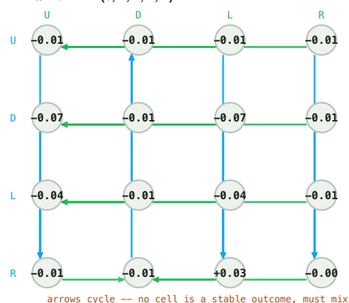
Q matrix -- (0, 1, 2, 1, 1)
