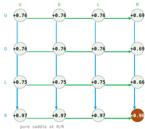
Q matrix -- (4, 2, 0, 2, 0)
