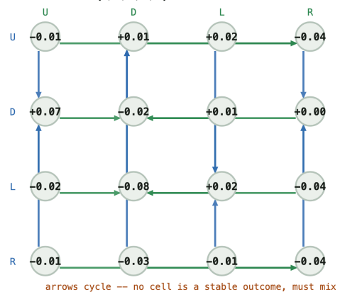
Q matrix -- (2, 3, 3, 3, 1)
