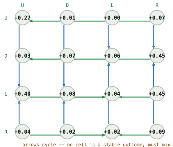
Q matrix -- (1, 3, 1, 4, 1)
