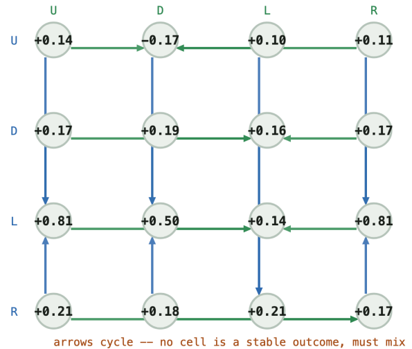
Q matrix -- (1, 1, 1, 0, 1)
