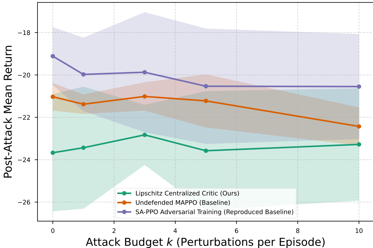
Robustness vs. Attack Budget ( \epsilon = 0.05 )
