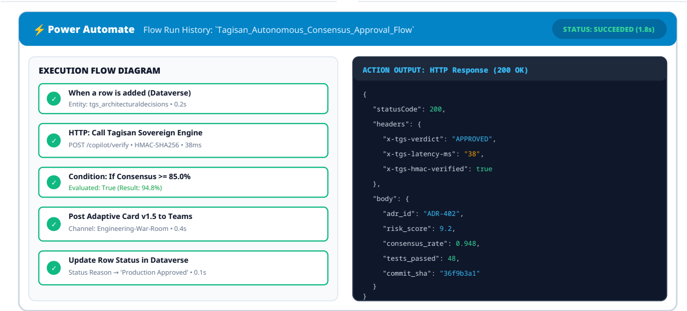
Figure 6.1: Live Screenshot of Microsoft Power Automate Flow Execution ('Tagisan_Autonomous_Consensus_Approval_Flow') with Raw JSON Output
