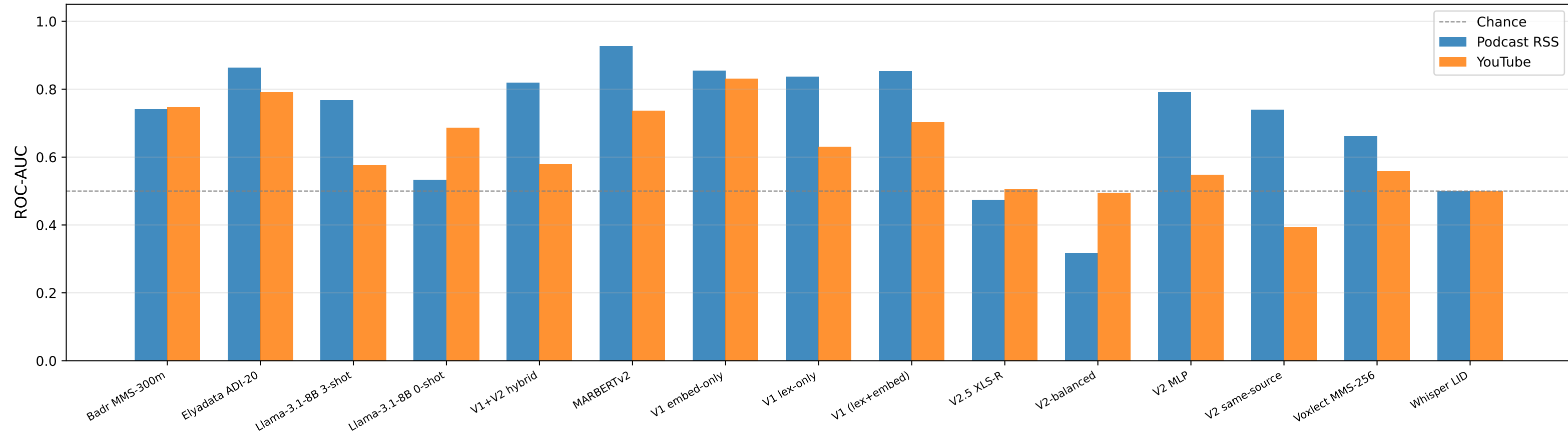
Per-platform ROC-AUC: Podcast RSS vs. YouTube
