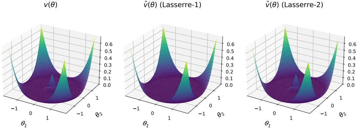
Figure 5: The true value function v(\theta) for the inverse kinematics problem (left) and the neural network’s learned approximation \hat{v}(\theta) trained on the first-order Lasserre (Shor) relaxation (center) and the tighter second-order Lasserre relaxation (right), over target positions \theta = (\theta_1, \theta_2) . Notably, the first-order Lasserre relaxation is not exact, and the neural network trained on it underestimates the true value function in the region inside the reachable annulus. The second-order Lasserre relaxation is exact, and the neural network trained on it closely matches the true value function.
