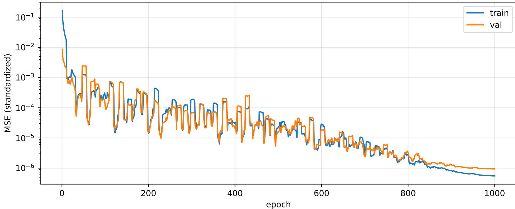
Training History (QCQP Example, Fold 0)
