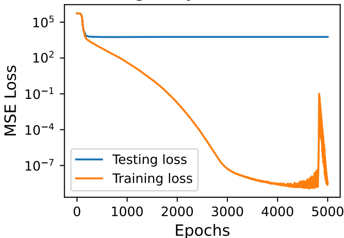
Training 6-layer FCN for SDP
