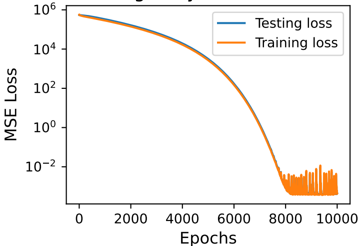
Training 6-layer ICNN for SDP
