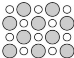
LiCl crystal
