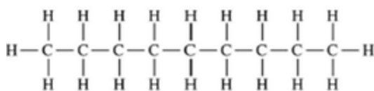
Nonane
