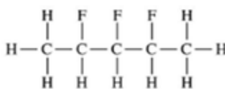
2,3,4-trifluoropentane
