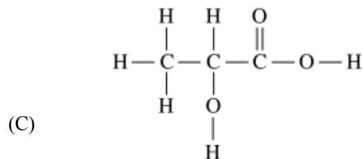
Lactic acid (90 g/mol)
