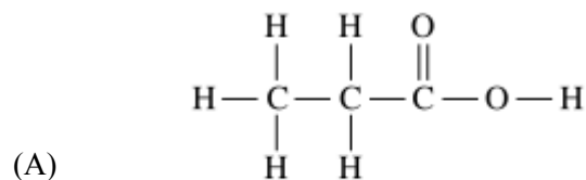
Propanoic acid (74 g/mol)
