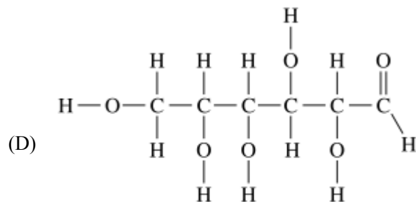
Glucose (180 g/mol)
