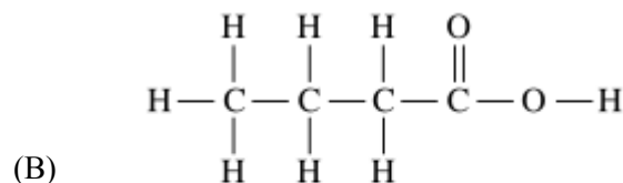
Butanoic acid (88 g/mol)
