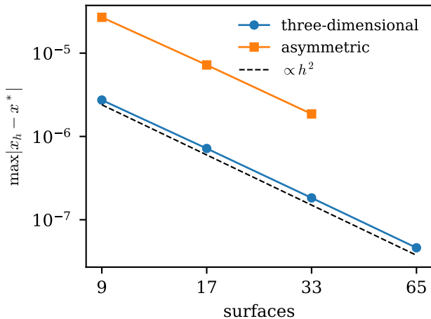
(a) manufactured mappings
