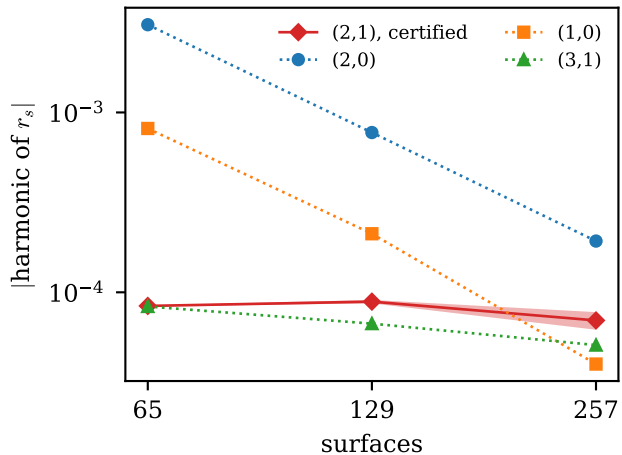
(b) rippled tokamak, \iota = 1/2
