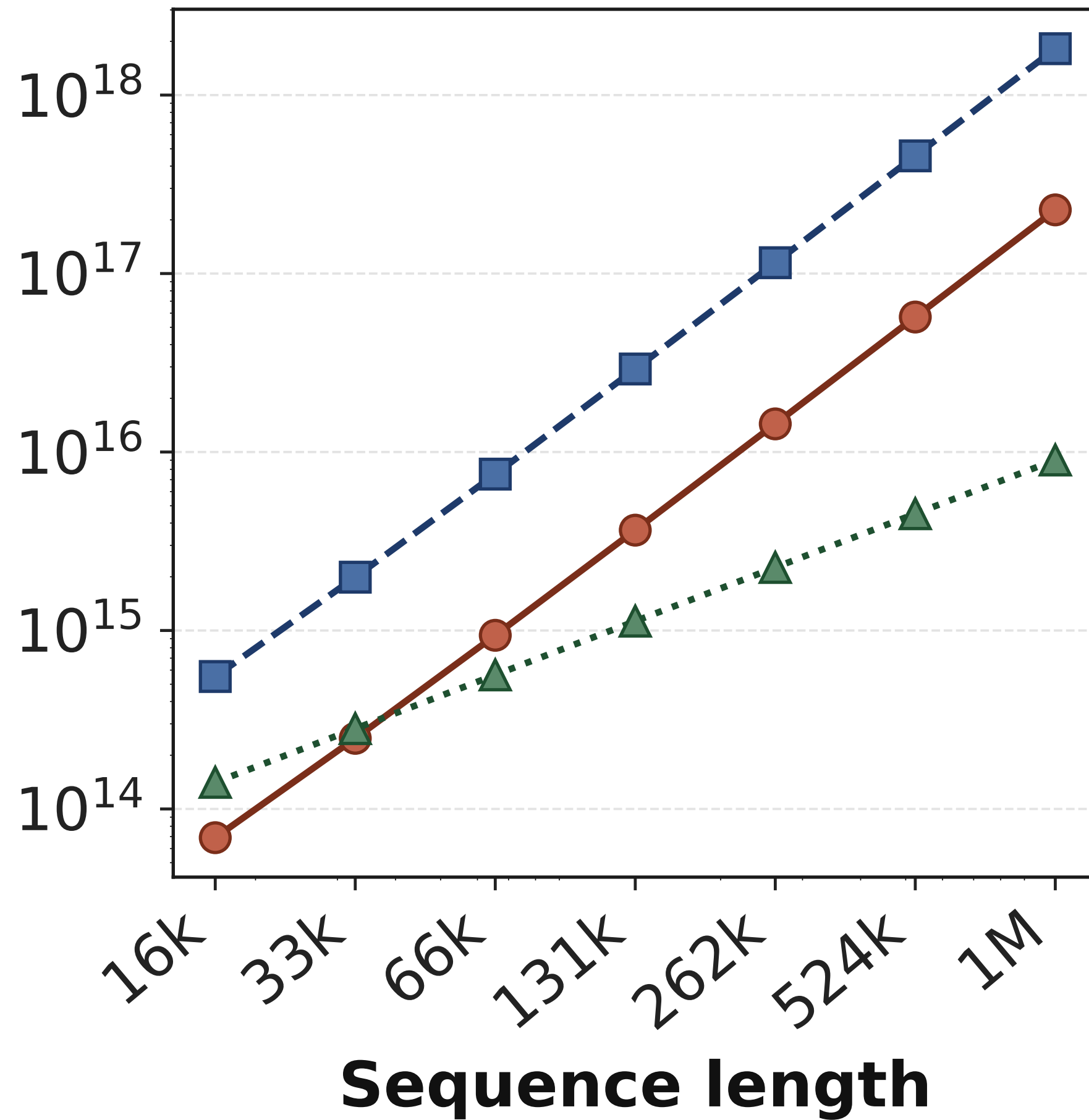
Attention FLOPs / sequence
