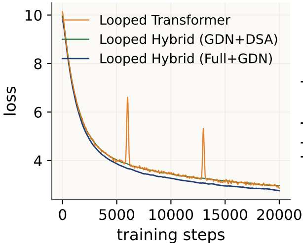
Language-modeling loss
