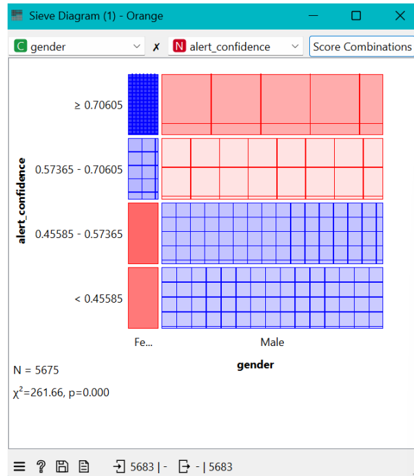
Figure 9: Sieve Diagram of Gender vs. Confidence
