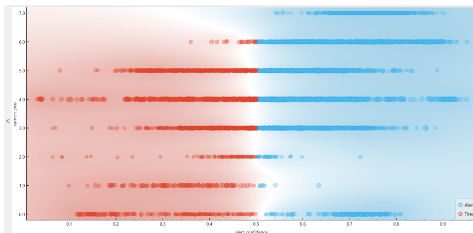
Figure 13: Camera Position vs Model Confidence of Classifications
