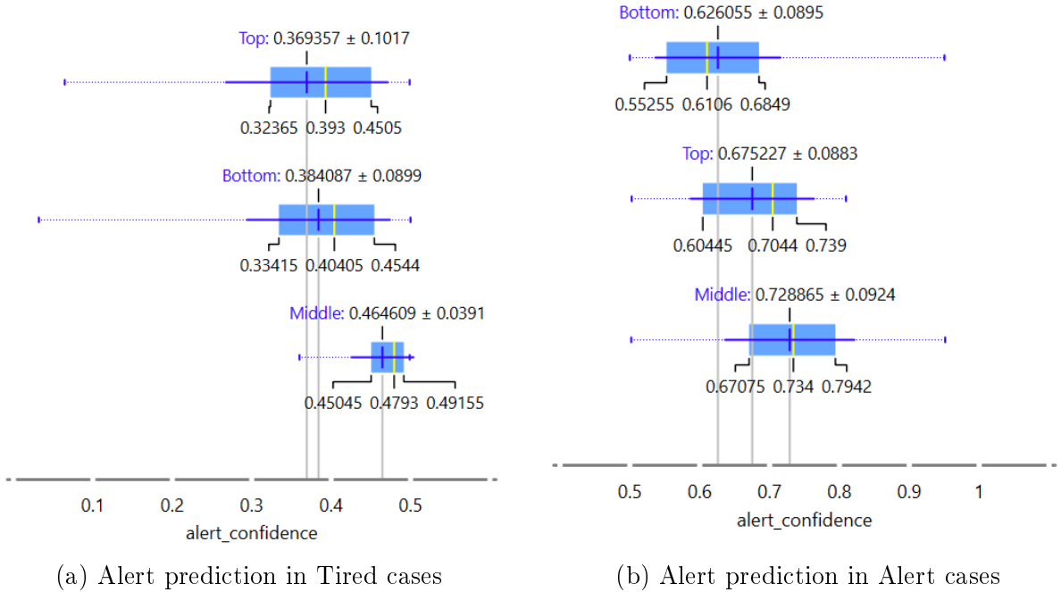
Figure 15: Positive predictions accross the camera locations
