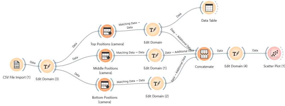
Figure 14: Camera Position separation
