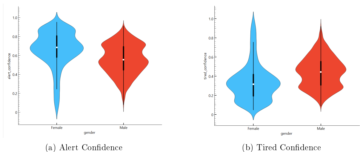
Figure 10: Comparison of model confidence scores by gender.
