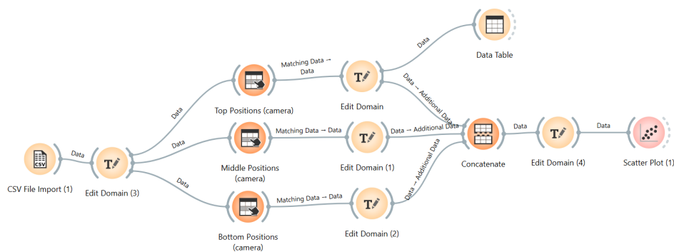
Figure 16: Camera Position separation
