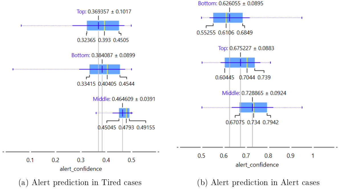
Figure 17: Positive predictions across the camera locations
