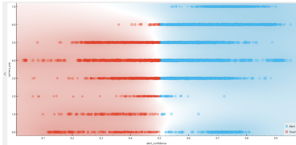
Figure 15: Camera Position vs Model Confidence of Classifications
