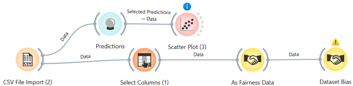
Figure 14: Node structure for fairness testing
