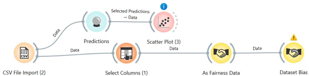
Figure 16: Node structure for fairness testing
