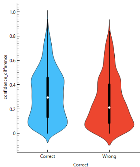
Figure 22: Distribution of Peak Classification Confidence vs Accuracy
