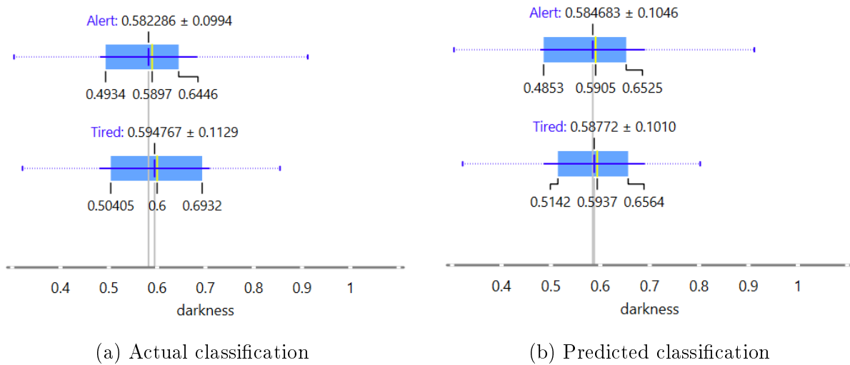
Figure 8: Comparison of darkness variance between actual and predicted classifications.
