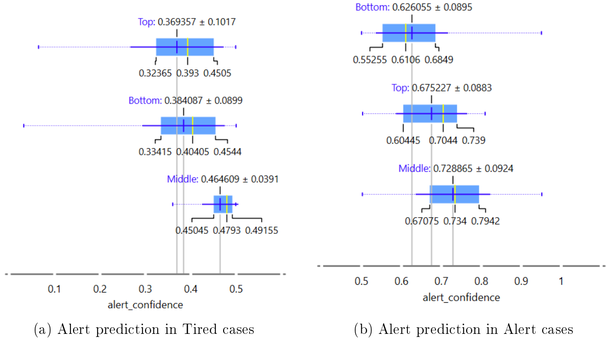
Figure 13: Positive predictions across the camera locations
