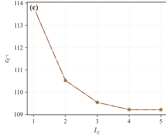
C^1 Error Bound
