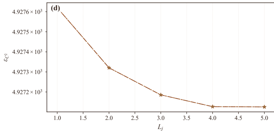
C^2 Error Bound
