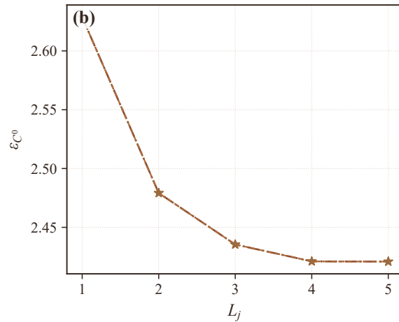
C^0 Error Bound
