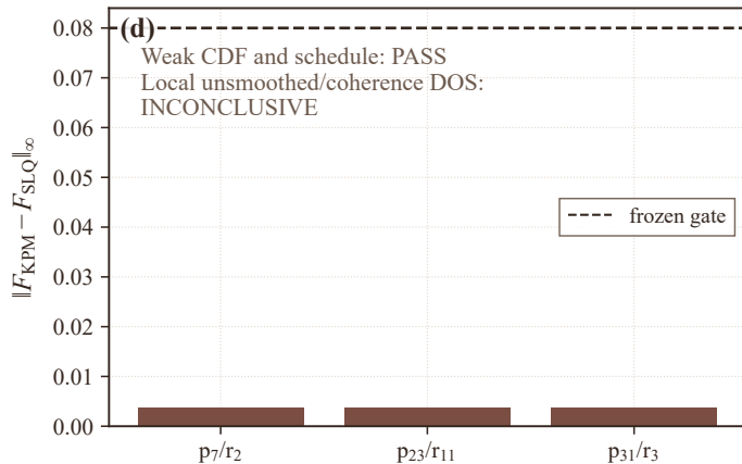
Method-Disagreement Bound
