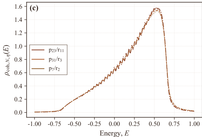
Coherence-Weighted Density
