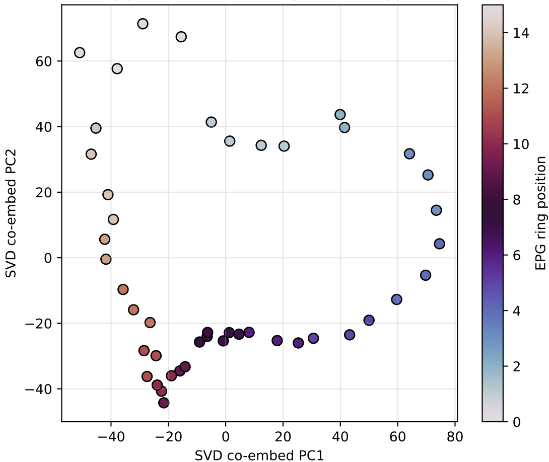
[epg] SVD co-embedding (one cell type)
