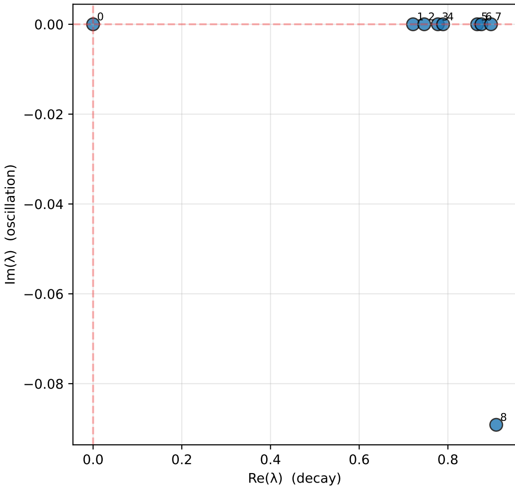
[d7epg] slow eigenvalues of L
