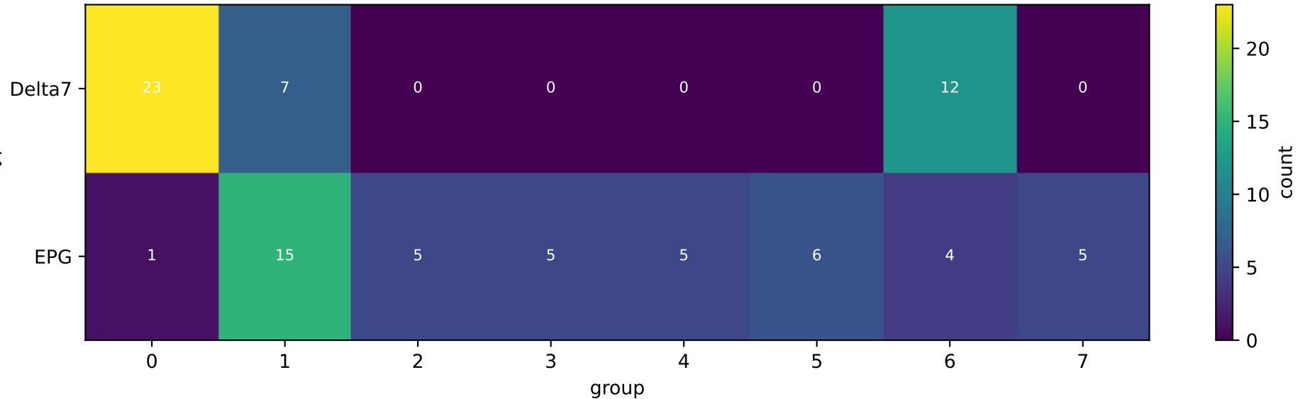
[d7epg] cell type x group (mean purity 0.92)
