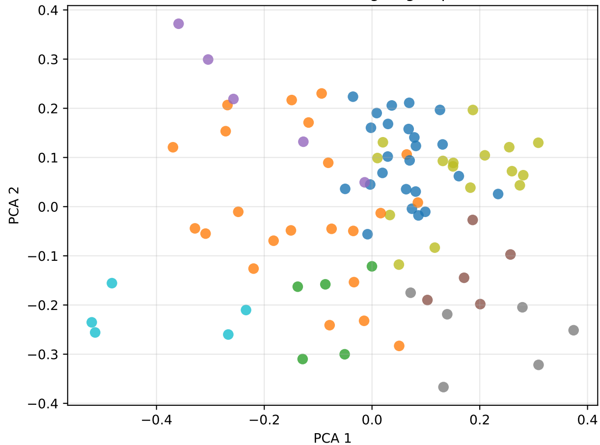
PCA of bi-embedding — group
