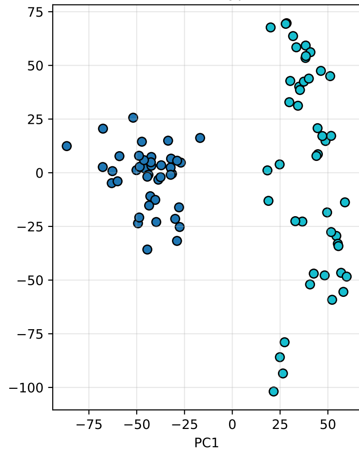
SVD of A K=2 ARI vs cell type = 1.00
