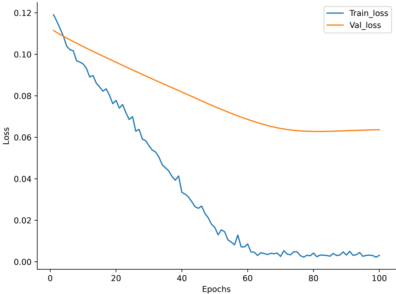
Loss curve
