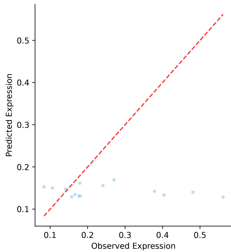
Baseline ctPred Pearson r = -0.2832
