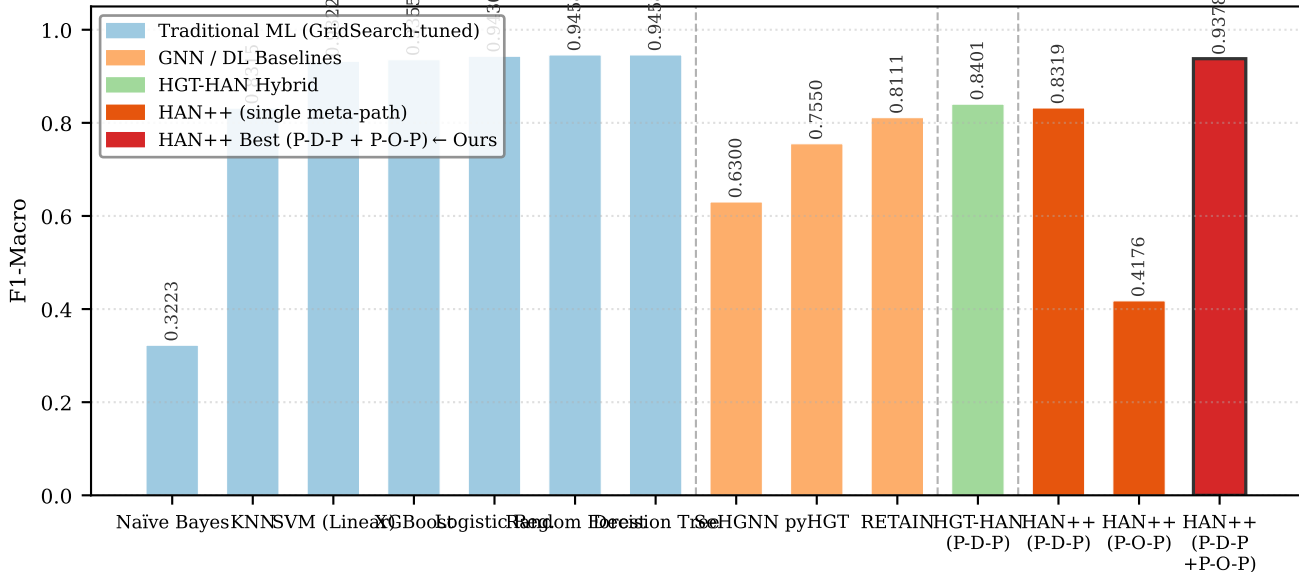
F1-Macro Comparison Across All Model Families (n = 48,546)
