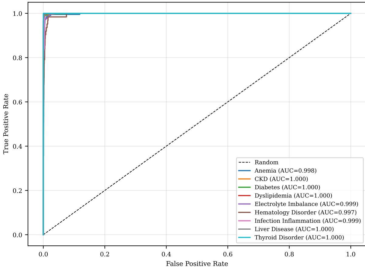
ROC Curves — Per Disease (Test Set)
