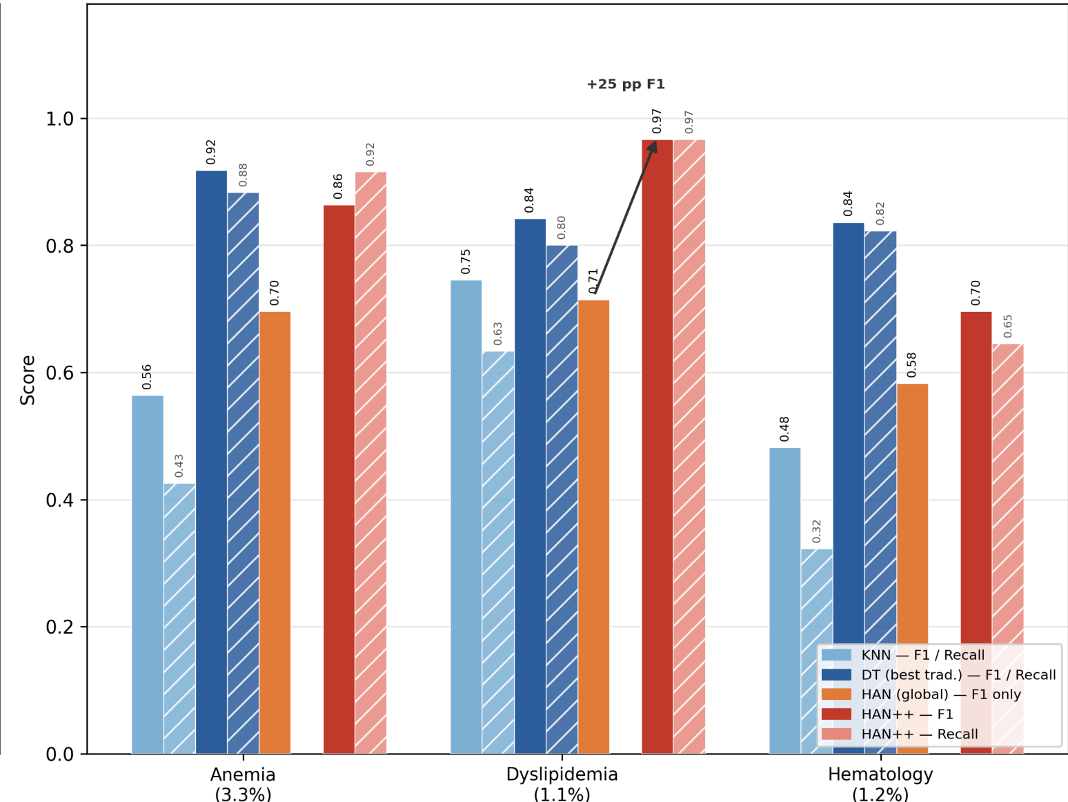
(b) Rare Disease Performance — F1 (solid) & Recall (hatched)
