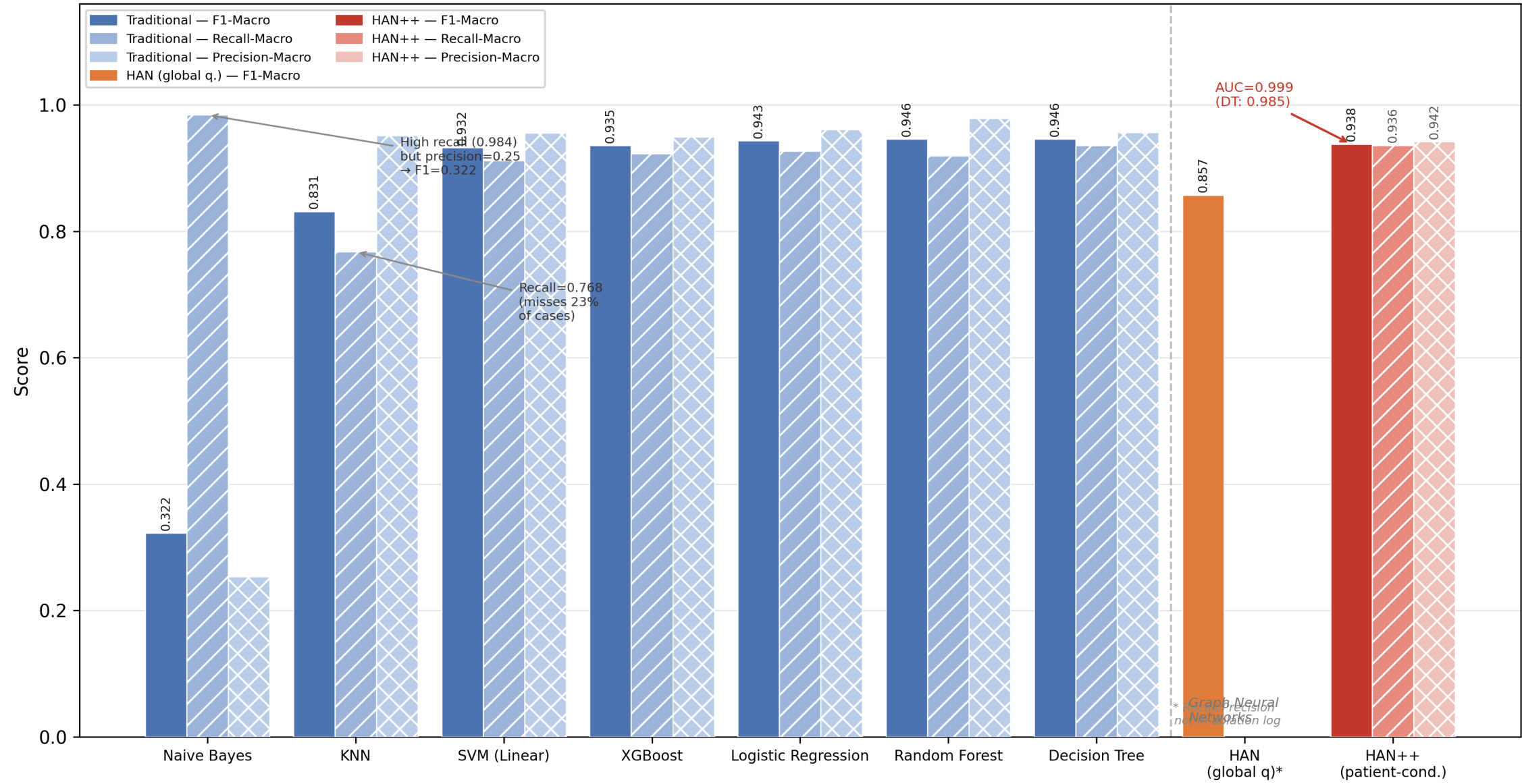
(a) Overall Performance: F1-Macro, Recall-Macro & Precision-Macro
