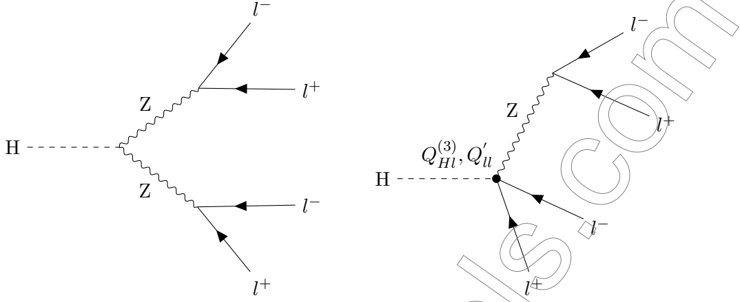
Figure 2.25: LO Feynman diagram for the H \rightarrow 4l decay in the SM (left) and a new diagram from \mathcal{L}_6 (right) with a hZll vertex that is generated by the Q_{Hl}^{(3)} and Q'_{ll} operators.
