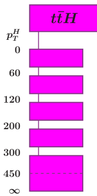
Figure 2.16: Stage 1.2 binning for the t\bar{t}H production mode in the STXS.
