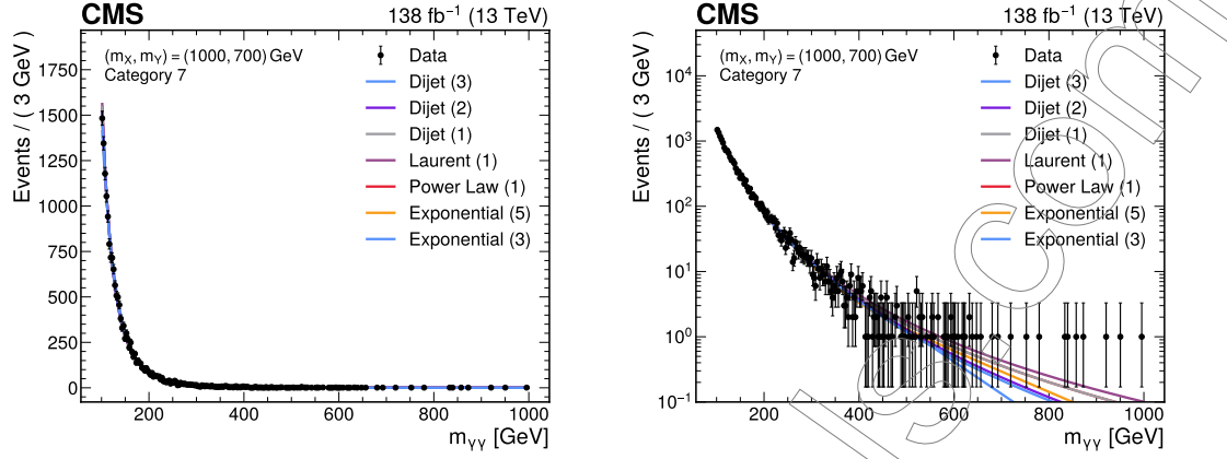
Figure 5.51: Envelope construction for the (m_X, m_Y) = (1000, 700) GeV mass point in the X \rightarrow Y(\gamma\gamma)H(\tau\tau) search. Shown is the m_{\gamma\gamma} distribution in data for a category consisting of the events passing preselection but not passing the pNN selection. The functions entering the envelope are indicated in the legend and their fits to the m_{\gamma\gamma} distributions are shown in the plots. The same plot is shown with a linear (left) and log (right) y-scale.
