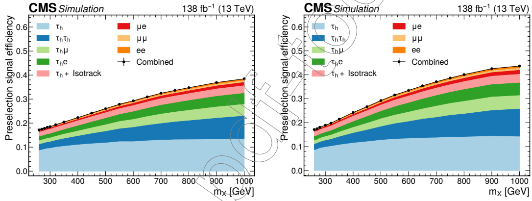
Figure 5.5: Preselection signal efficiency as a function of m_X in the X^{(0)} \rightarrow HH (left) and X^{(2)} \rightarrow HH (right) searches. The contributions from the different channels are shown by the stacked filled histograms and the combined efficiency shown by the black points. The statistical uncertainty in the combined uncertainty is plotted but is too small to be seen.
