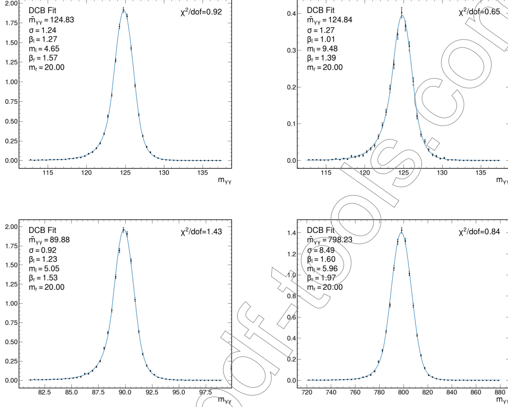
Figure 5.39: DCB fits in category 0 in 2018 for the X \rightarrow Y(\tau\tau)H(\gamma\gamma) search (top) and X \rightarrow Y(\gamma\gamma)H(\tau\tau) search (bottom). The mass points are (m_X, m_Y) = (600, 90) (top-left), (300, 70) (top-right), (600, 90) (bottom-left), and (1000, 800) GeV (bottom-right).
