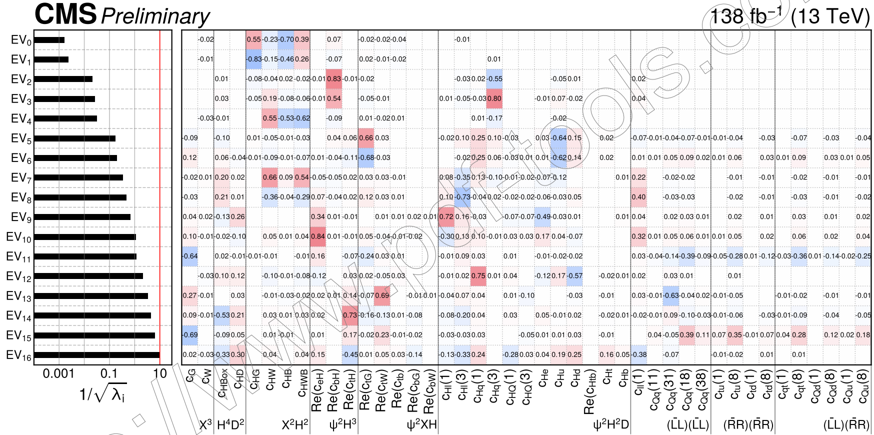
Figure 6.9: The rotation matrix, \mathcal{R} , derived using the PCA procedure, truncated according to the 17 eigenvectors included in the fit to data. The values in the matrix are shown by text and a colour scale that goes from blue (negative values) to red (positive values). The left panel shows the expected 68% CL interval given by 1/\sqrt{\lambda_i} , where \lambda_i is the eigenvalue for eigenvector i .
