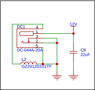
12V DC_IN
