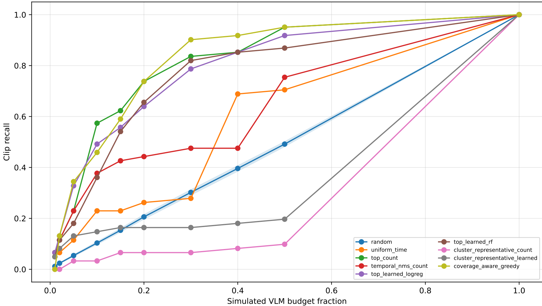
Clip recall at event gap 4s
