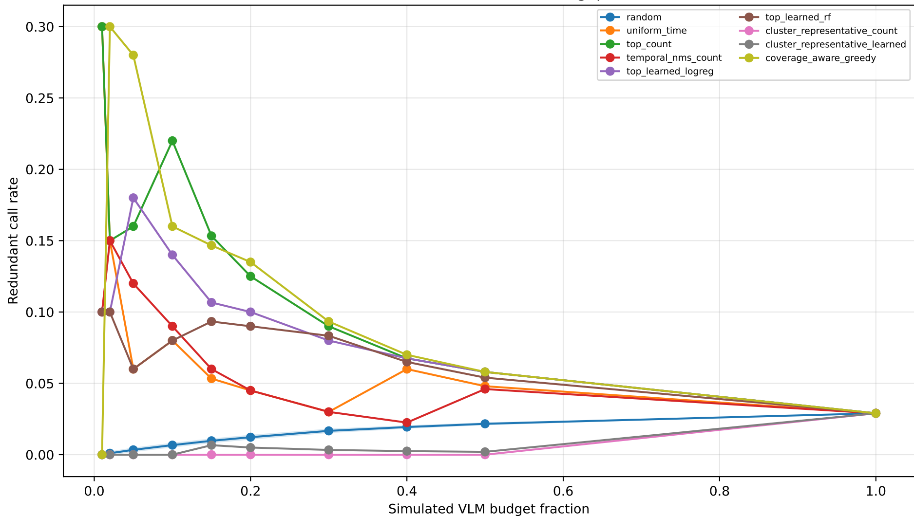
Redundant call rate at event gap 4s
