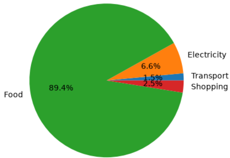
Emission Share
