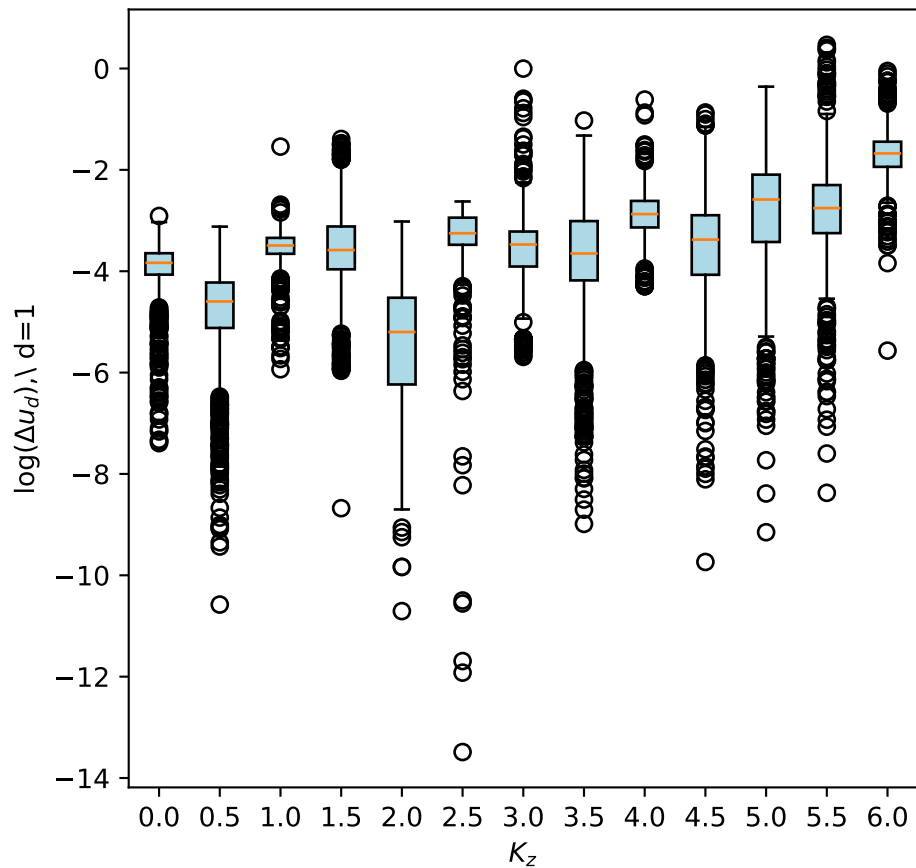
log-errors in u(x) v/s K_z
