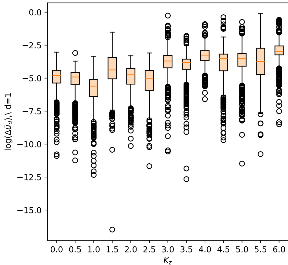
log-errors in \bar{u}(x) v/s K_z
