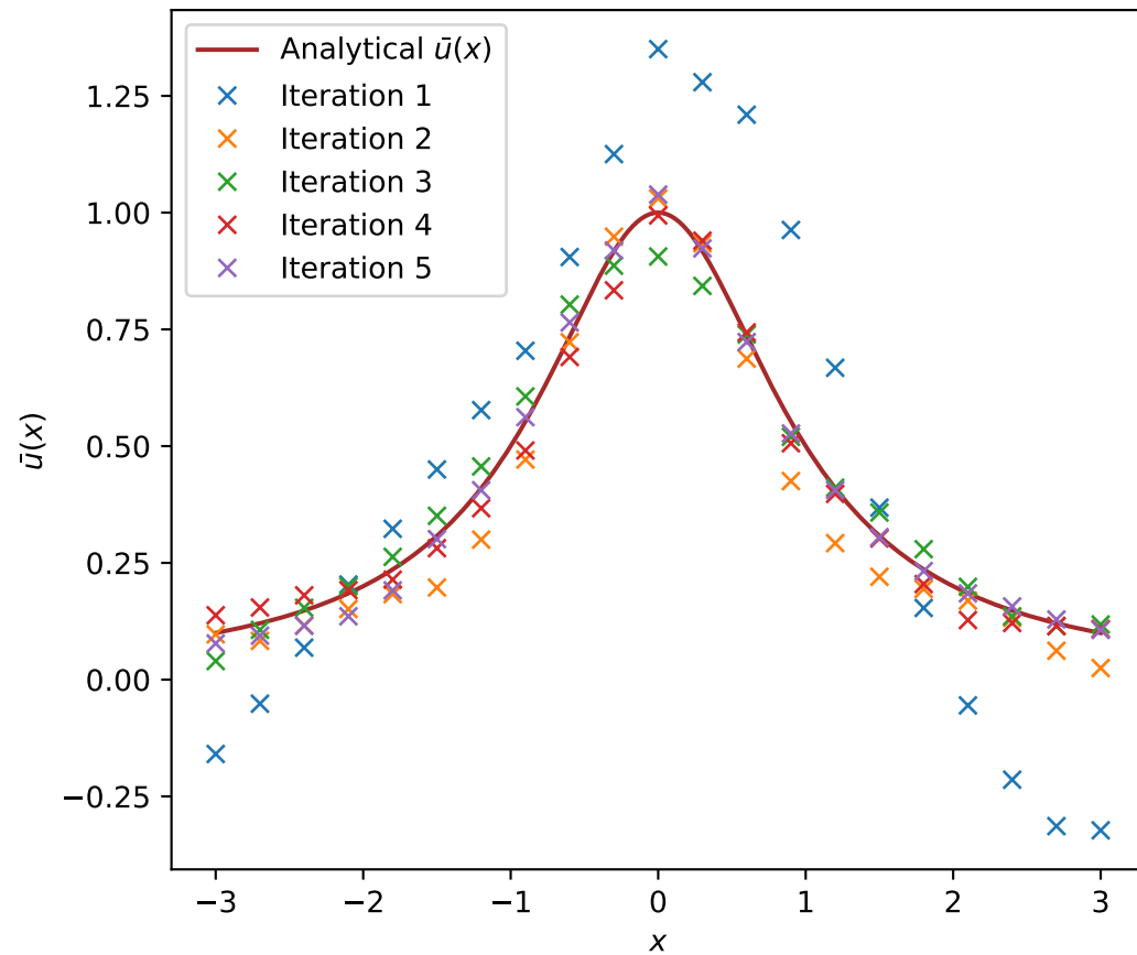
\bar{u}(x)
