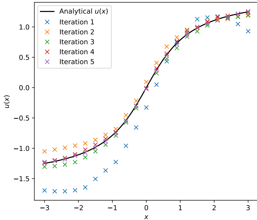
u(x)
