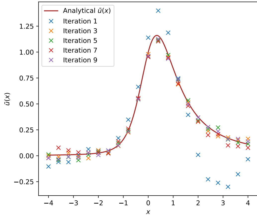
\bar{u}(x)
