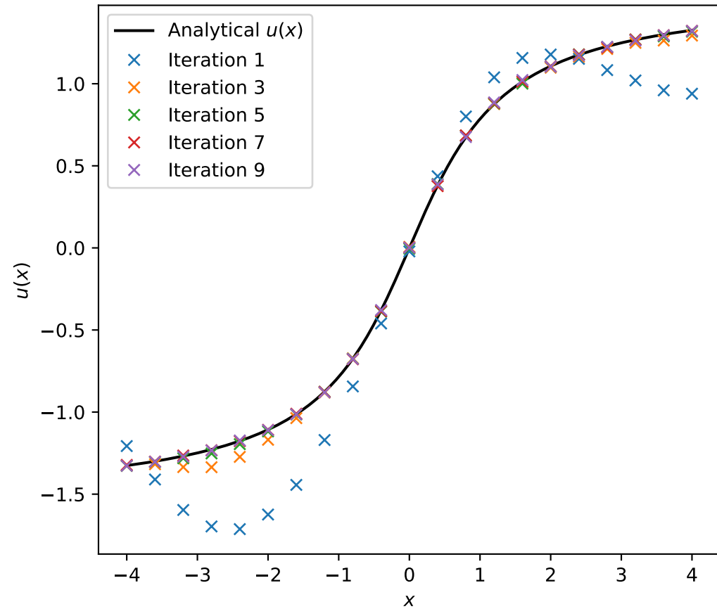
u(x)
