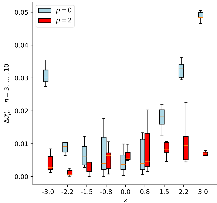
Errors in \bar{u}(x) for different p
