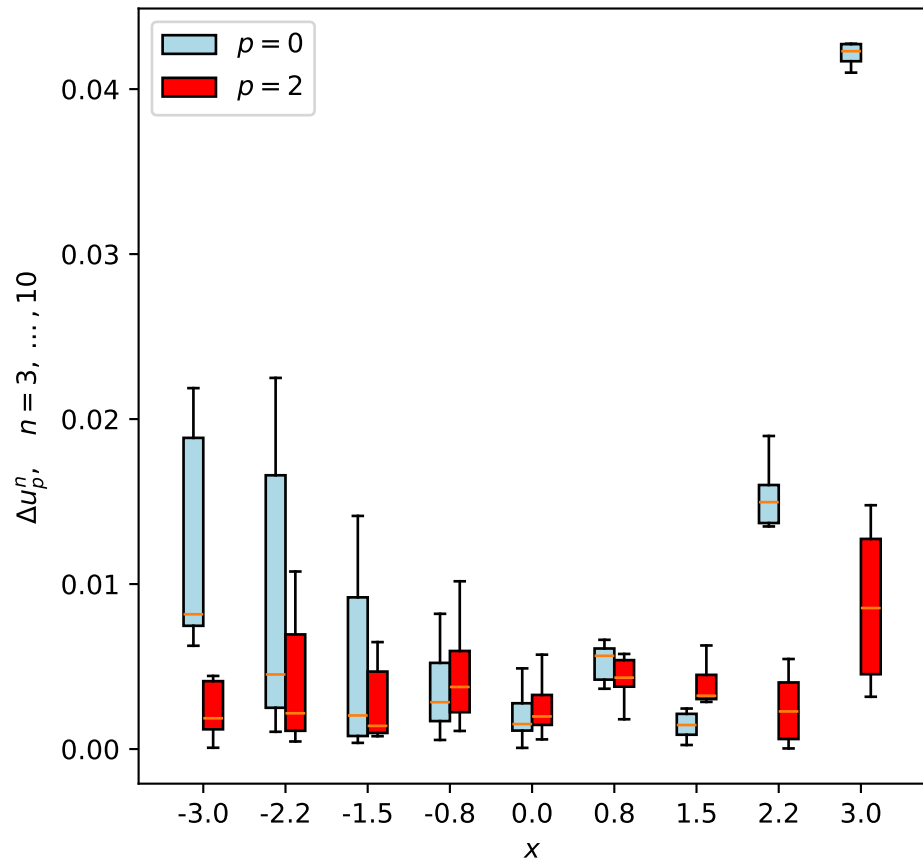
Errors in u(x) for different p
